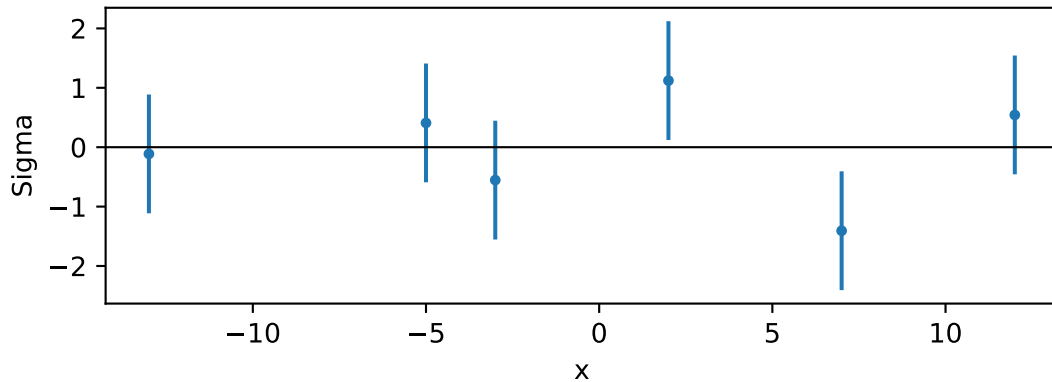
\sigma Residuals for fit example
